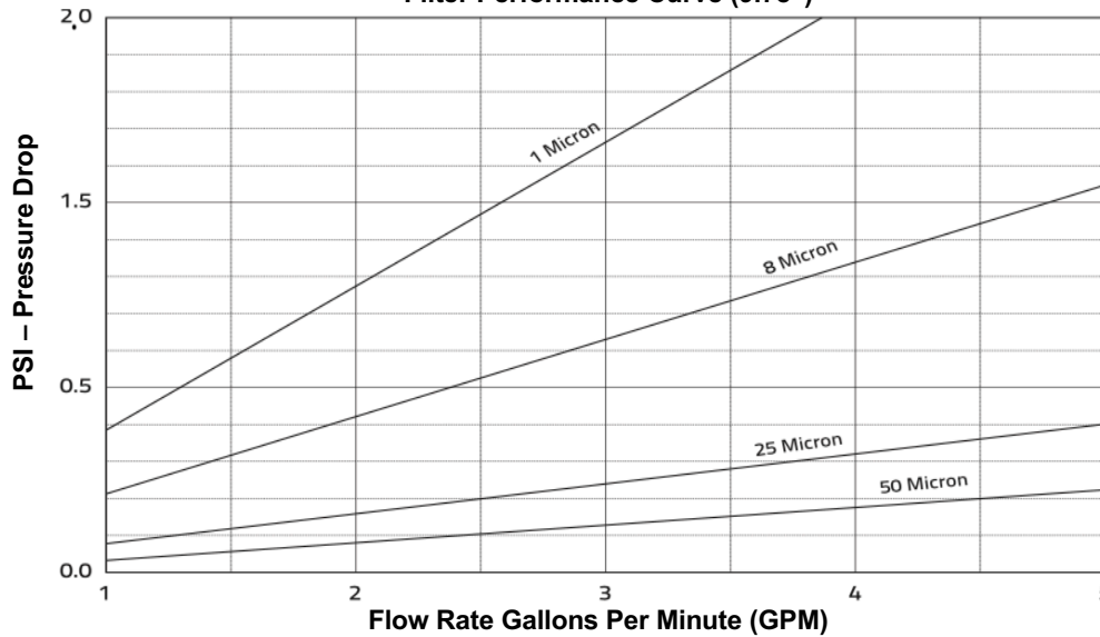
Filter Performance Curve (9.78")
